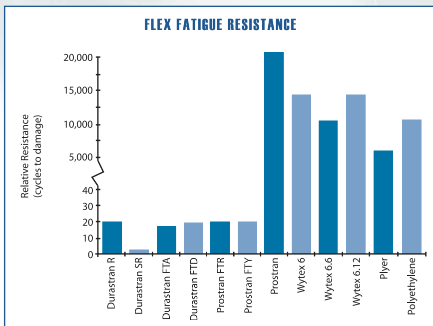
FLEX FATIGUE RESISTANCE (Cycles to Damage)
